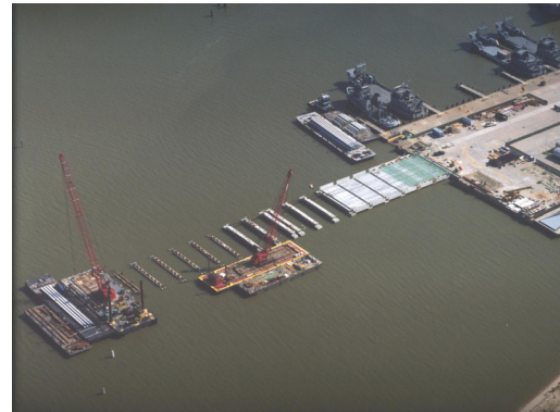
Driving concrete piles and setting precast concrete pile caps
